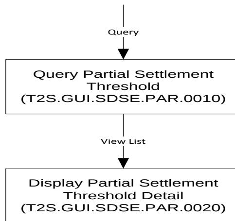
Figure 4-59 Partial Settlement Threshold Query user interface framework
