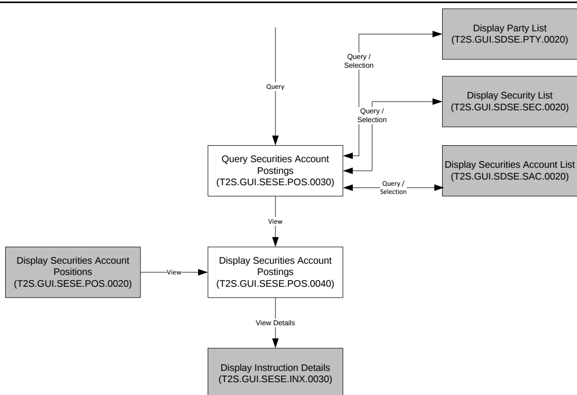
Figure 2-5 Securities Account Postings user interface framework
