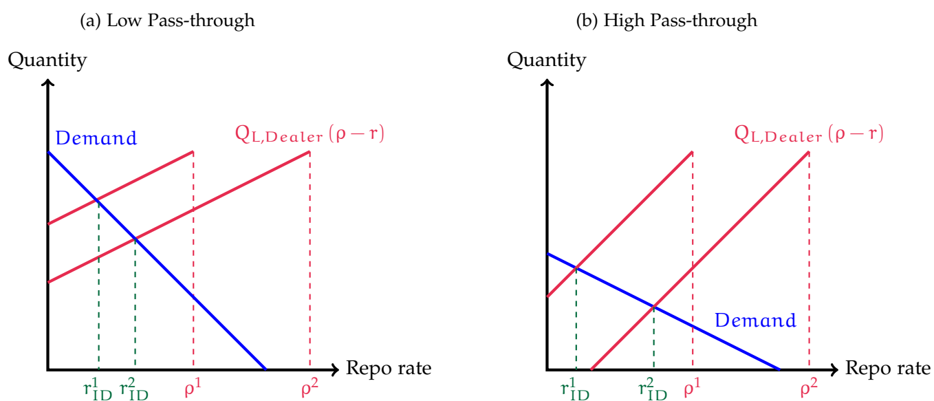
Figure IA.3: DFR - ID Pass-through Intuition
