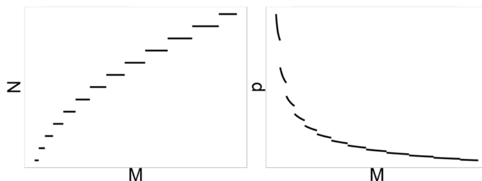
Figure IA.2: Dealer relationship number and prices with endogenous link formation
