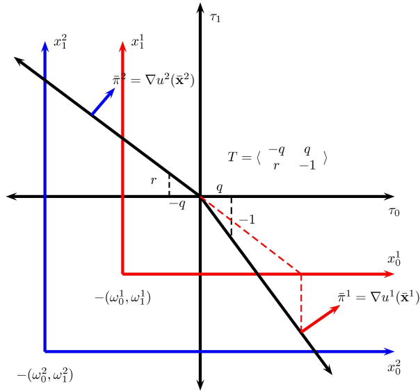
Figure 2: Competitive borrowing and lending with bankruptcy. What was the net transfer space before now gets a kink. Optimality for the lender requires that his utility gradient \pi^l is orthogonal to the ray spanned by the vector T^l = (-q, r) . For the borrower the utility gradient \pi^s is orthogonal to the ray spanned by T^s = (q, -1) because he holds a short position in the bond. The default penalty is equal to the vertical distance of his optimal decision point to the point where his date one consumption is zero. The equilibrium problem is that q and r have to adjust such that the linear space spanned by T^l = (-q, r) passes through the time 1 zero consumption point of agent 1. At this point the real net transfers are such that they add up to zero.
