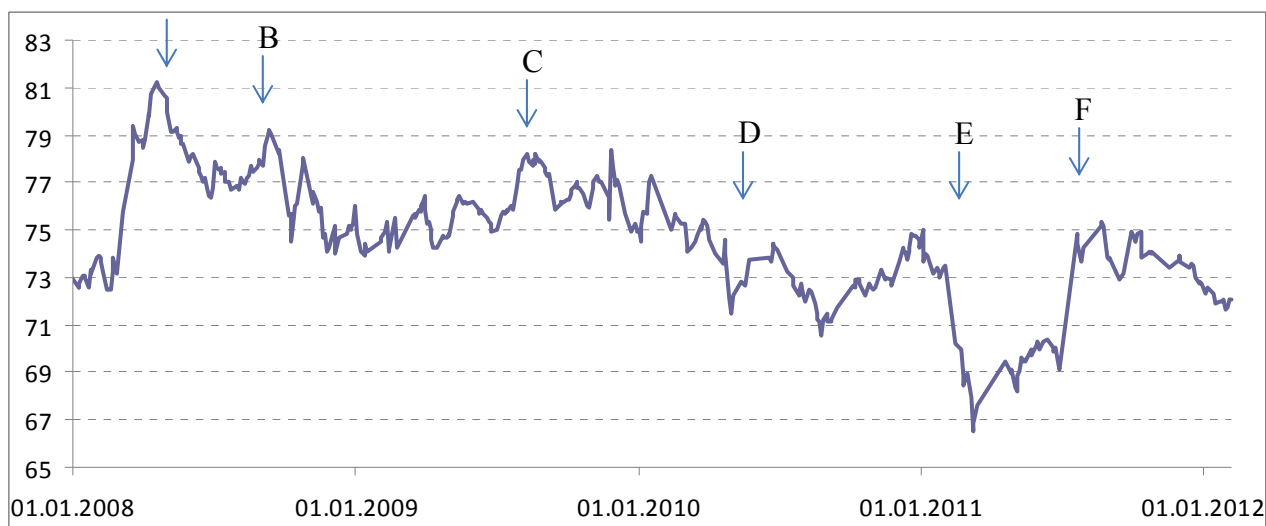
Figure 4. Total spillover plot, 200-day window, 10-steps-ahead forecast, January 2008- February 2012.
