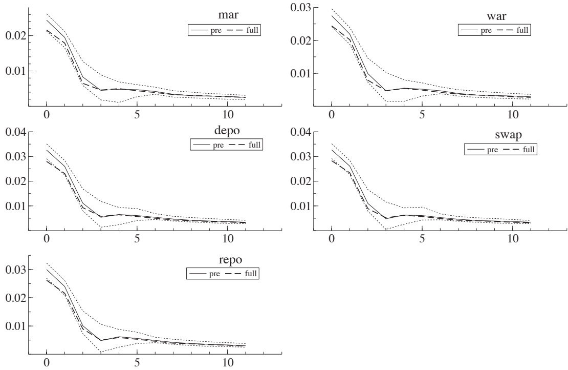
Figure 3: Impulse responses of interest rate spreads to common shock
